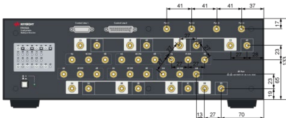
Dimensions (front view, E5092A with option 020, in millimeters)
