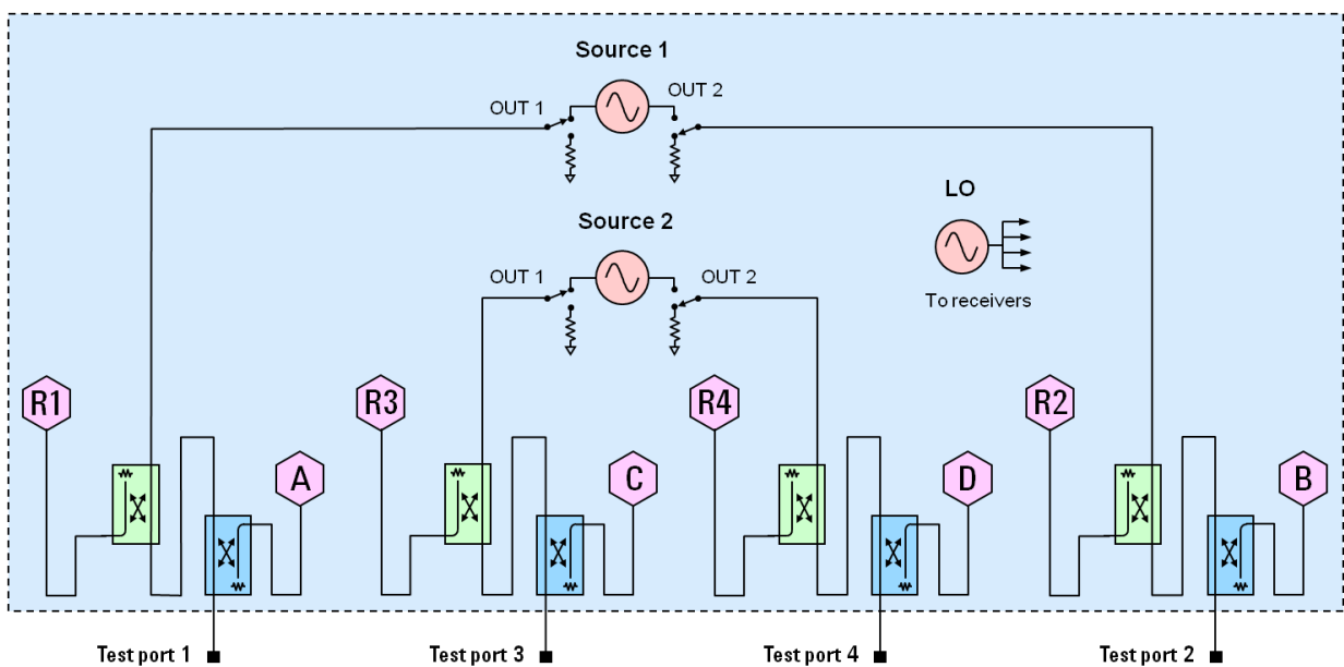
Figure 2. N5224B and N5225B Option 410 (4-port metrology configuration)
