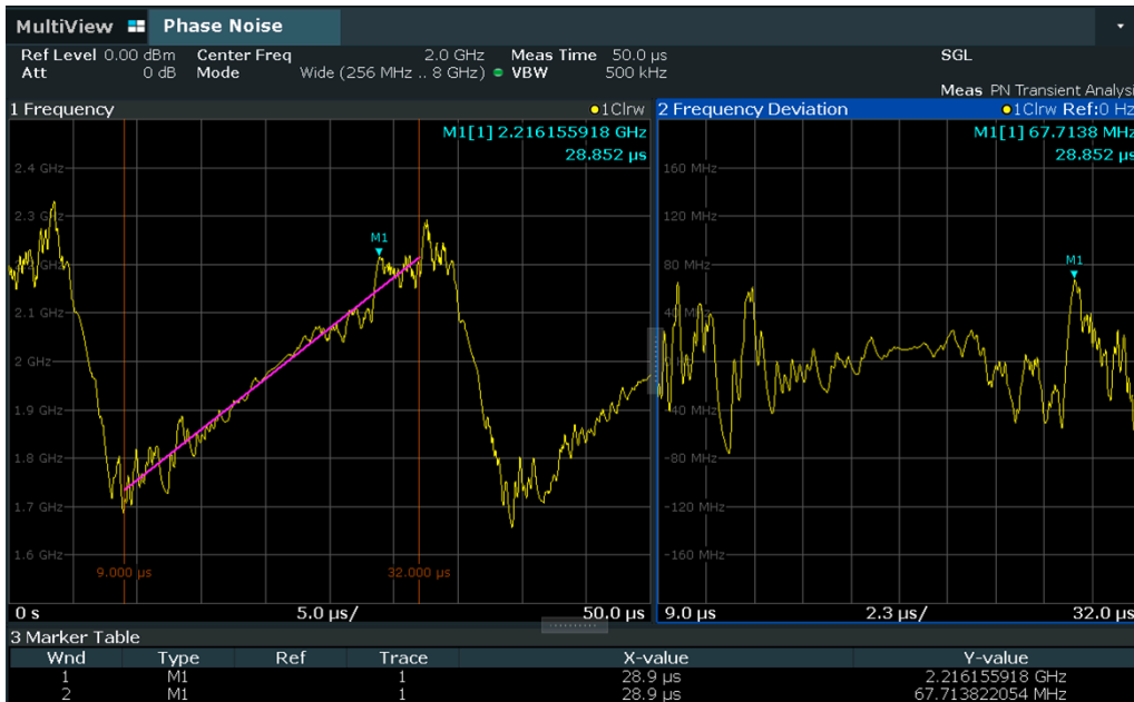
Linearity analysis of FMCW chirps. Left: the pink reference line is visible between the evaluation lines. Right: the deviation of the frequency from linear behavior is displayed.
