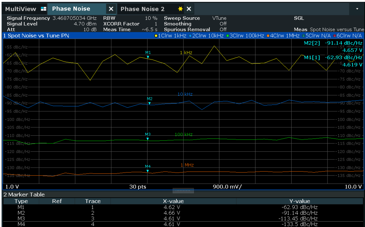
VCO phase noise at offset frequencies of 1 kHz, 10 kHz, 100 kHz and 1 MHz relative to the tuning voltages
