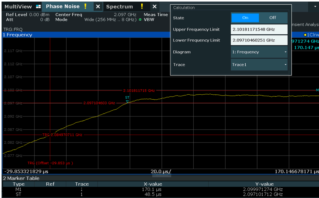
Automatic settling time measurement: after defining the tolerance frequency range, the settling time is displayed in the result summary.
