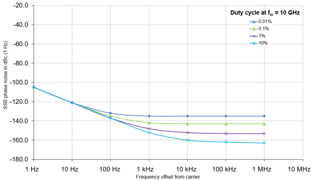
Typical AM noise sensitivity at f_{in} = 10 GHz (start offset = 1 Hz, cross-correlation factor = 1, signal level = 10 dBm, gating = on)
