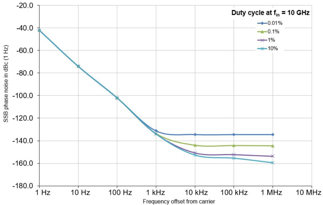
Typical phase noise sensitivity with R&S®FSWP-B60 or R&S®FSWP-B61 option at f_{in} = 10 GHz (start offset = 1 Hz, cross-correlation factor = 1, signal level = 10 dBm, gating = on)
