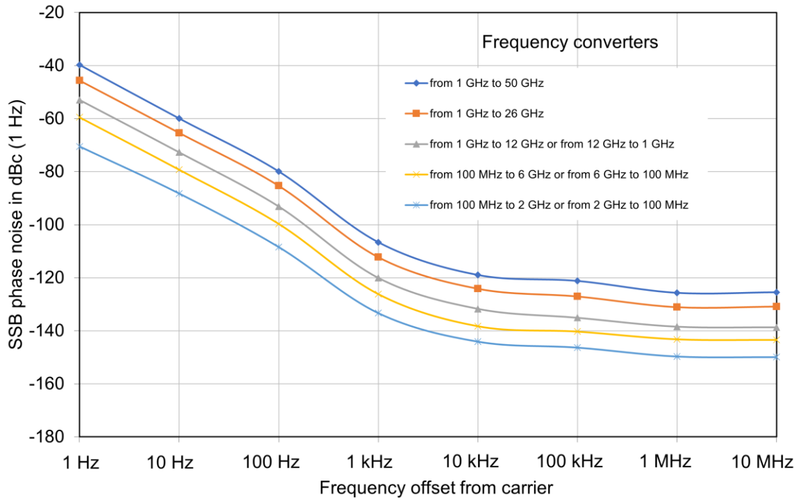
Typical phase noise sensitivity of frequency converter measurements with R&S®FSWP-B61 option (start offset = 1 Hz, cross-correlation factor = 10)
