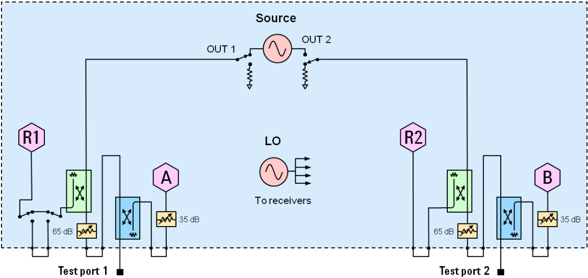
Figure 2. 2-Port N5244B and N5245B Option 217
