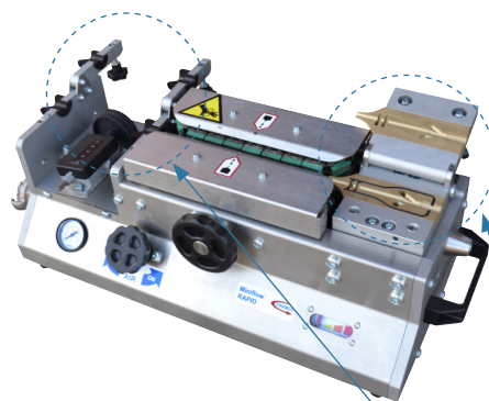
Configured machine with both inlet guides and adaptor plates. Ready to operate.
