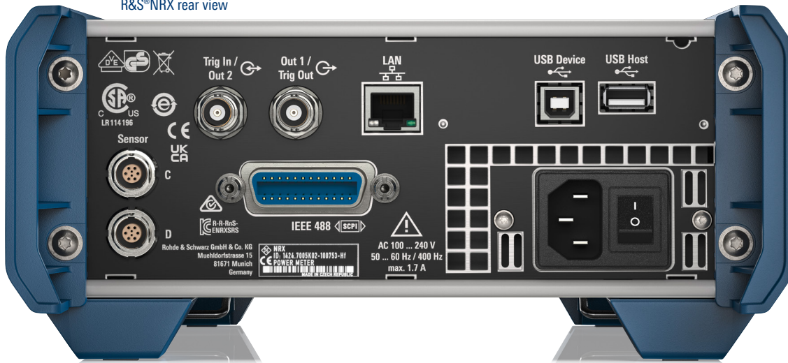
R&S®NRX rear view
