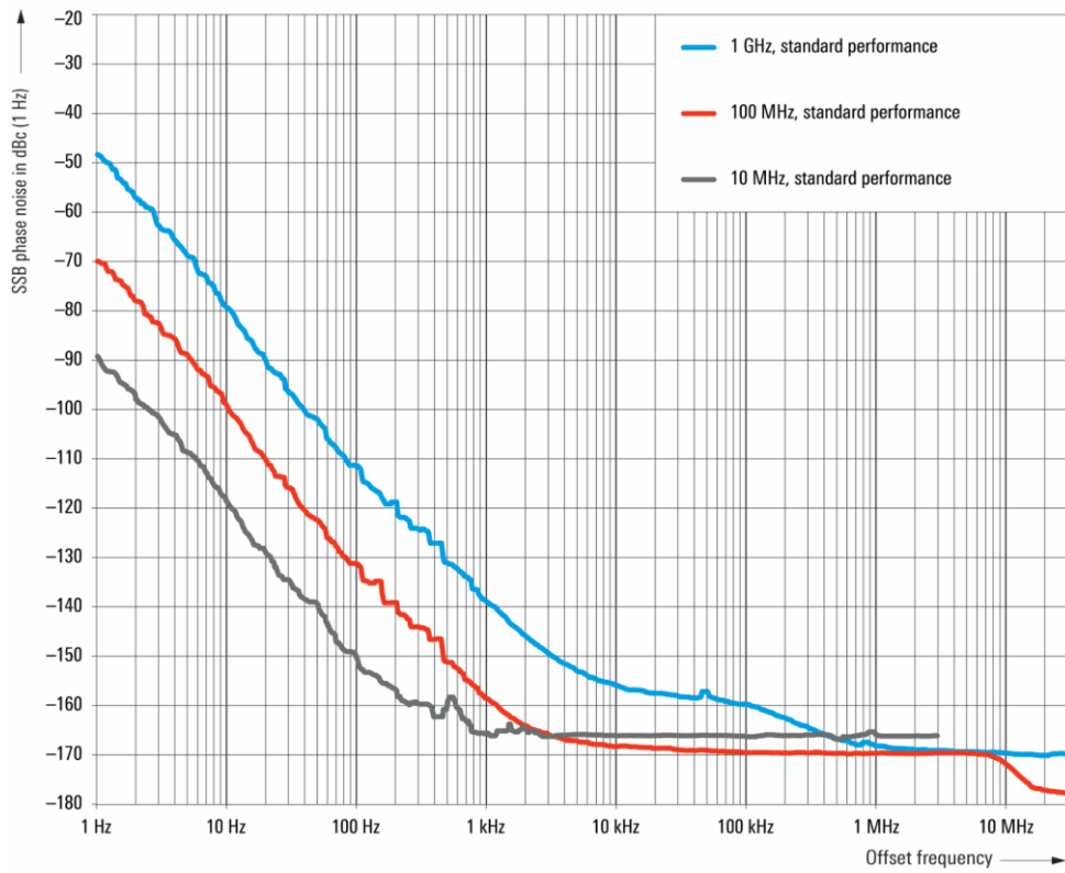
Measured SSB phase noise of reference outputs at f = 10\text{ MHz} , 100\text{ MHz} and 1\text{ GHz} ( f = 100\text{ MHz} and f = 1\text{ GHz} only available with the R&S ® SMAB-K703 option)
