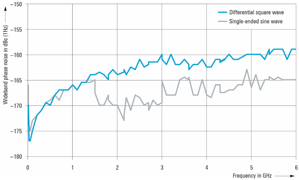
Measured wideband noise of clock synthesizer output at maximum output power versus carrier frequency with the R&S®SMAB-B29 and R&S®SMAB-K722 options. Measured with the R&S®FSWP phase noise analyzer and VCO tester
