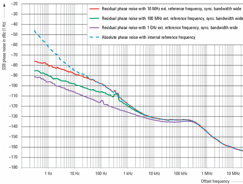
Measured residual SSB phase noise at f = 10 GHz with the R&S ® SMAB-B711 option; comparison of different reference frequencies against absolute phase noise
