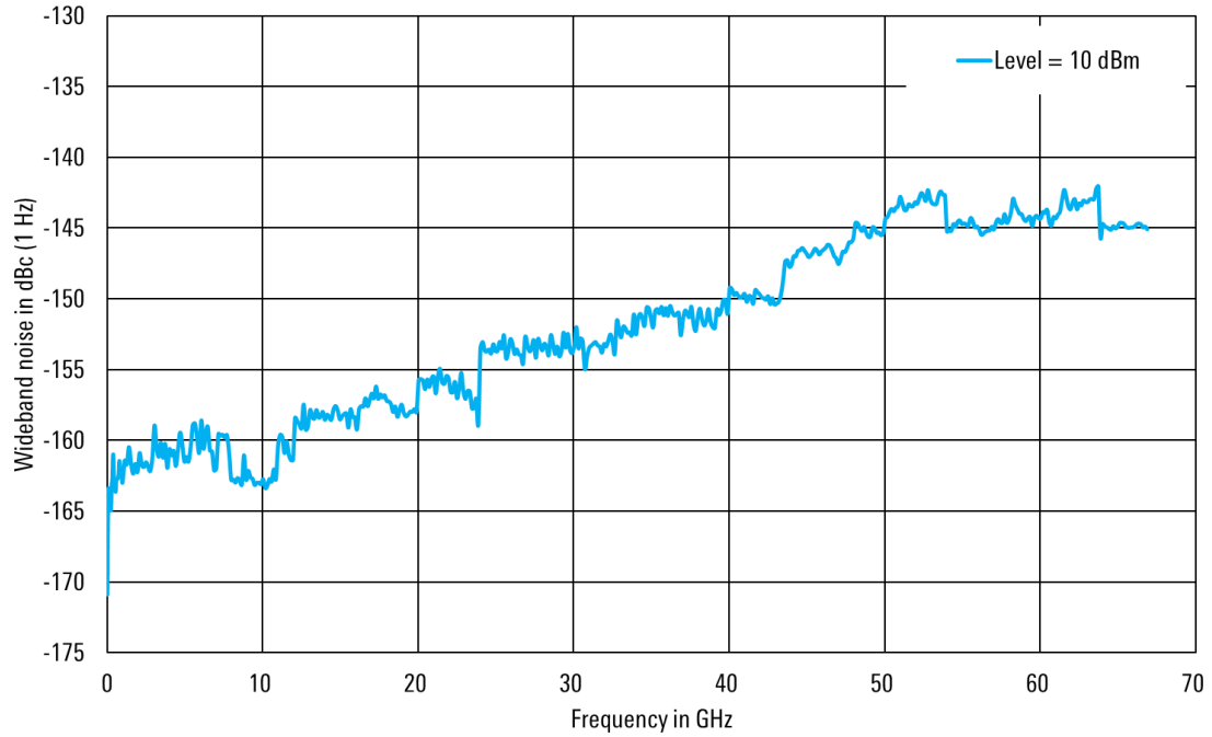
Measured wideband noise at 70 MHz offset and +10 dBm versus carrier frequency with the R&S ® SMAB-B167, R&S ® SMAB-B711 and R&S ® SMAB-B39 options. Measured with the R&S ® FSW85 signal and spectrum analyzer
