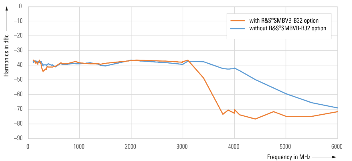
Measured harmonics second order, CW, level = +13 dBm
