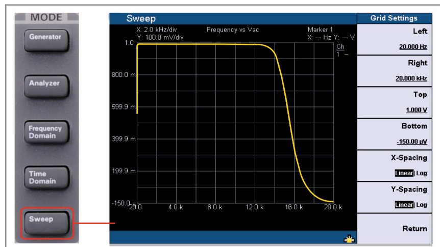
Figure 10. Use a single button to access the swept measurement mode.
