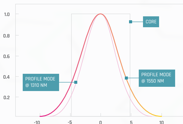
Pic.2b. MFD dependence on wavelength
