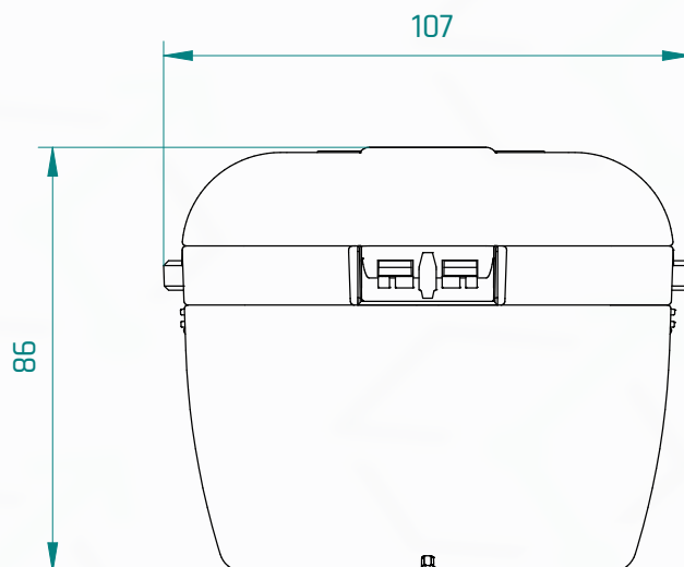
Pic1. The OSC dimensions
