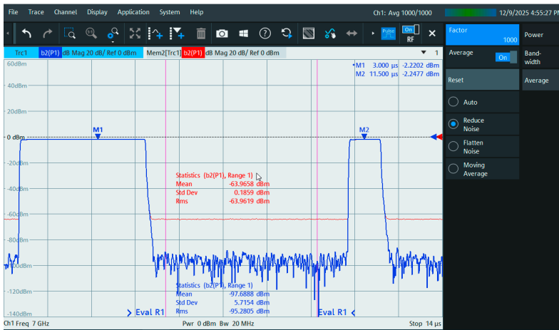
Pulse profile measurement: the wideband measurement mode enables single-shot pulse sweeps without averaging. Averaging (AVG) modes are also available to achieve either a very low trace noise or a very high dynamic range (i.e. a high pulse on/off ratio) based on vector averaging. Red trace: AVG mode "flatten noise". Blue trace: AVG mode "reduce noise".
