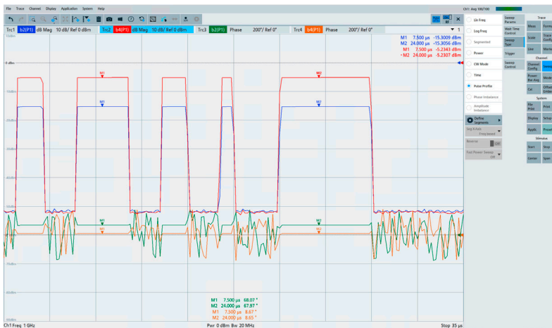
Pulse profile measurement with arbitrary pulse sequences. Pulse sequences can be measured on multiple receivers simultaneously. Since the receivers are phase coherent, they not only measure the amplitude of a pulse but also its phase with high stability. This allows the phase deviation of a DUT to be determined very simply and reliably.
