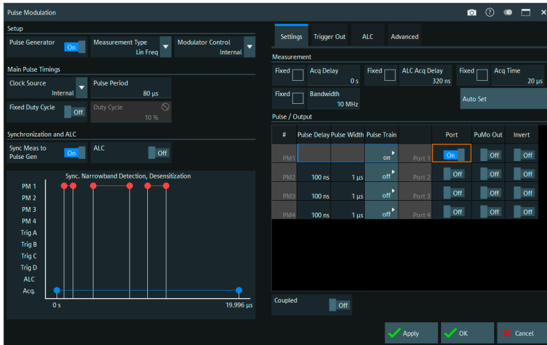
Configuration of parameters for pulsed signal measurements
