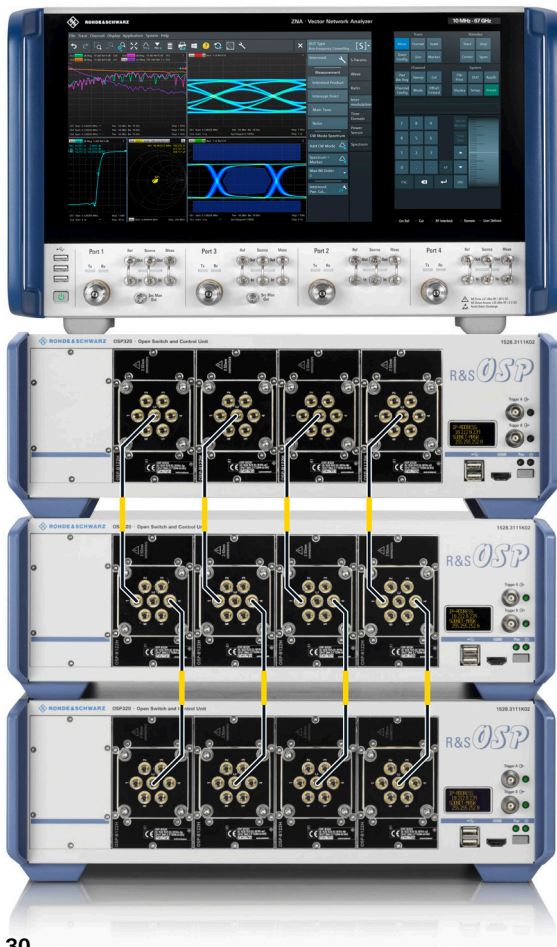
R&S®ZNA based multiport solution for fully automated multiport testing; highest flexibility is provided by integrating the configurable R&S®OSP320 open switch and control units.
