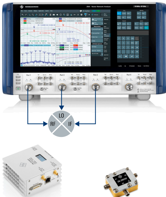
R&S®ZN-ZCG as phase reference
